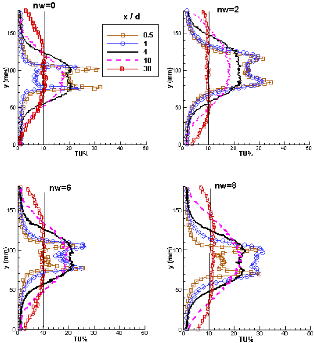
Figure 11 Normalized diagrams of turbulence intensity profiles in Re=10000 versus the sampling interval for the circular cylinder with different number of trip wires on its surface ( \frac{d}{D}=0.075 ) in all stations (nw is the number of wire sign)
