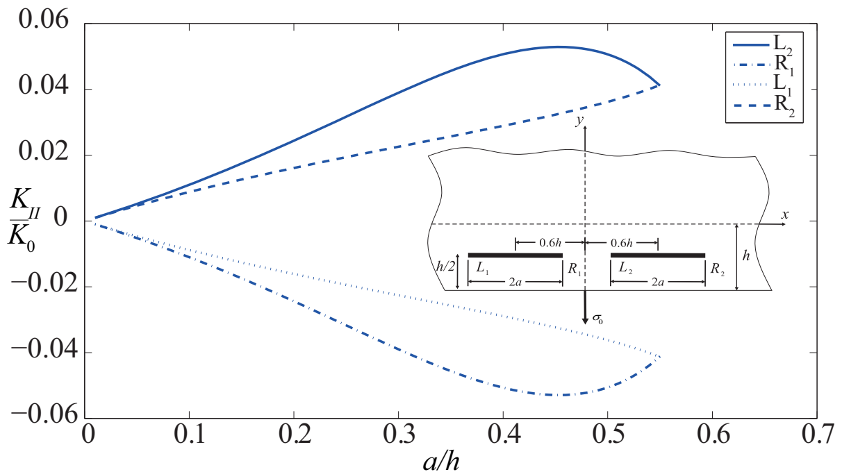
Figure 6 Non-dimensional mode II stress intensity factors for two collinear cracks.
