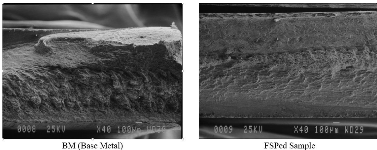
Figure 8 Fracture surface SEMs of FS and FS9 samples.
