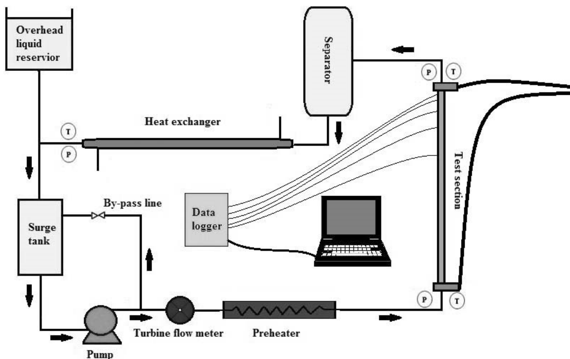
Figure 2 Schematic diagram of experimental loop.
