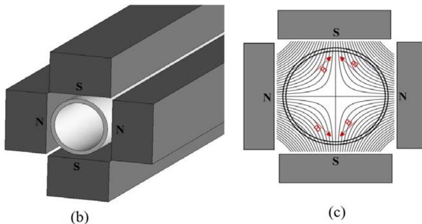
Figure 3 (a) Test section and thermocouple locations; (b) used quadrupole magnet; and (c) magnetic field lines.
